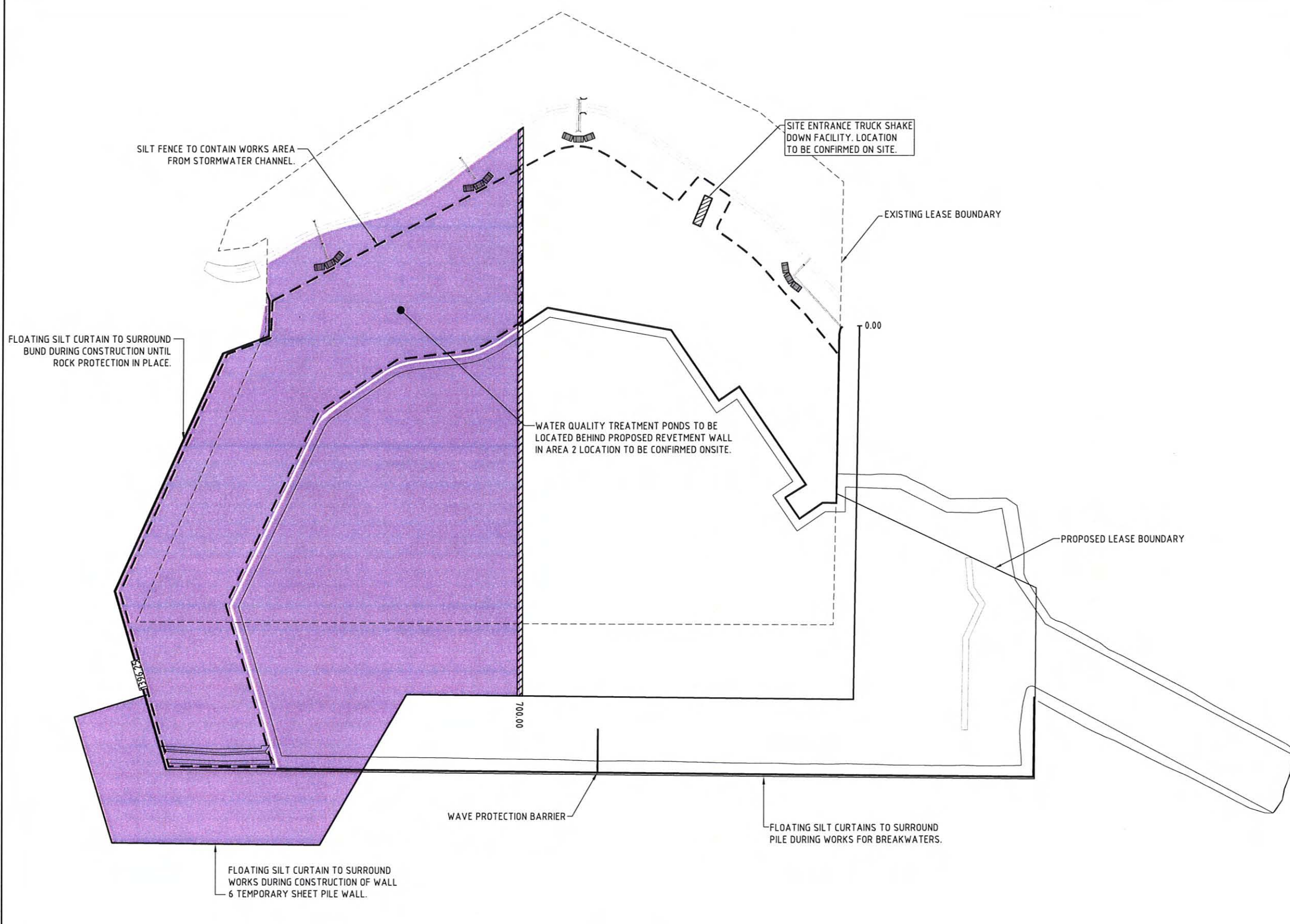
PHASE 3 PLAN SCALE 1:2000
