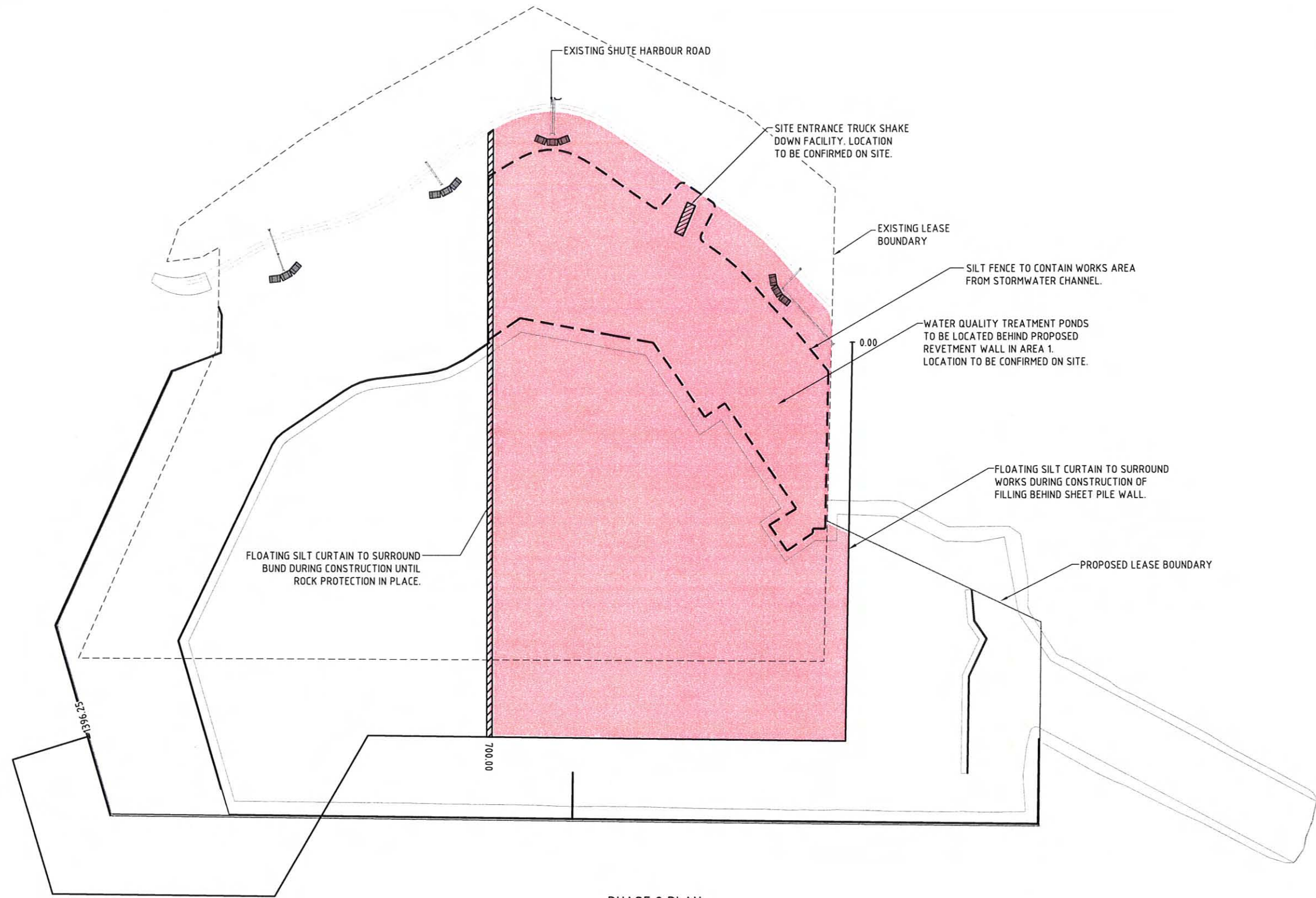
PHASE 2 PLAN SCALE 1:2000
